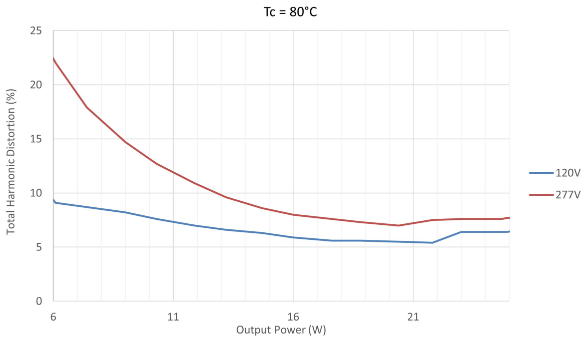
THD versus output power
