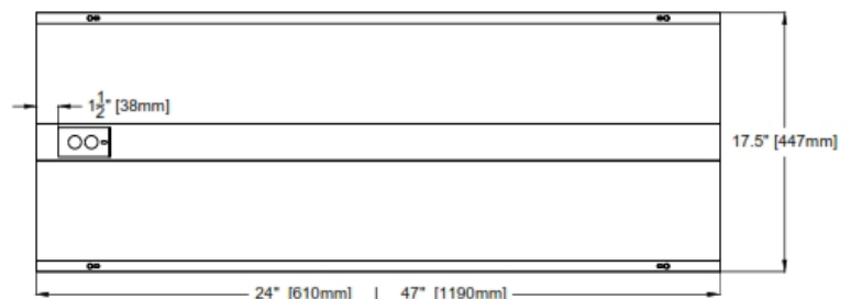
S HB-20 Base View
