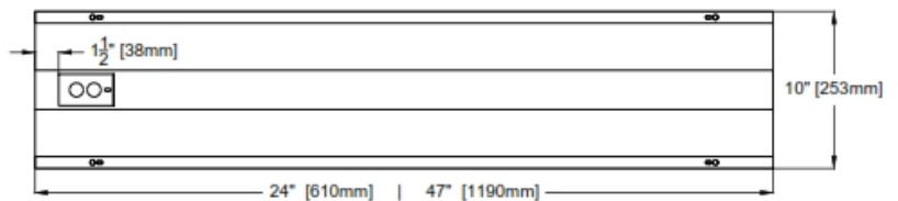
S HB-12 Base View
