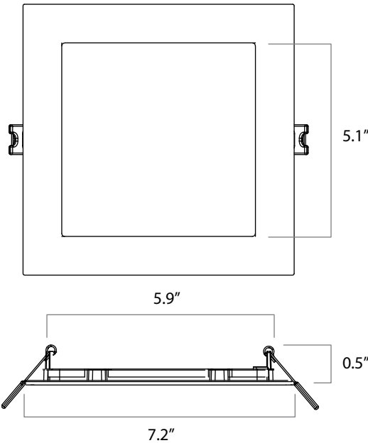
Downlight 6" Square
