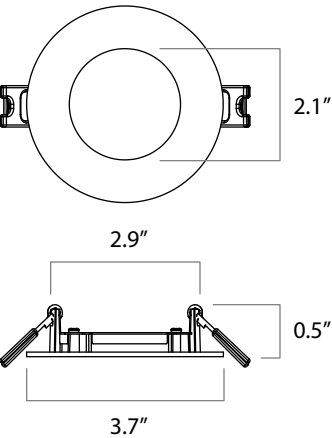
Downlight 4" Round
