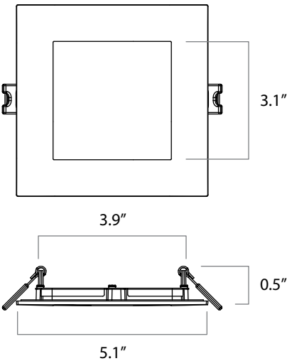
Downlight 4" Square
