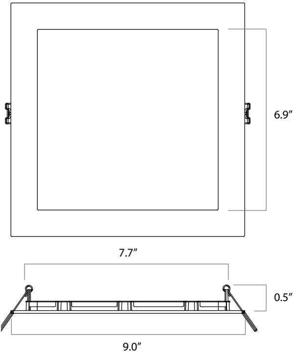
Downlight 8" Square
