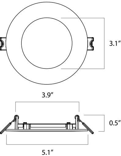
Downlight 4" Round
