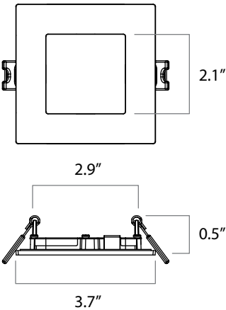
Downlight 4" Square
