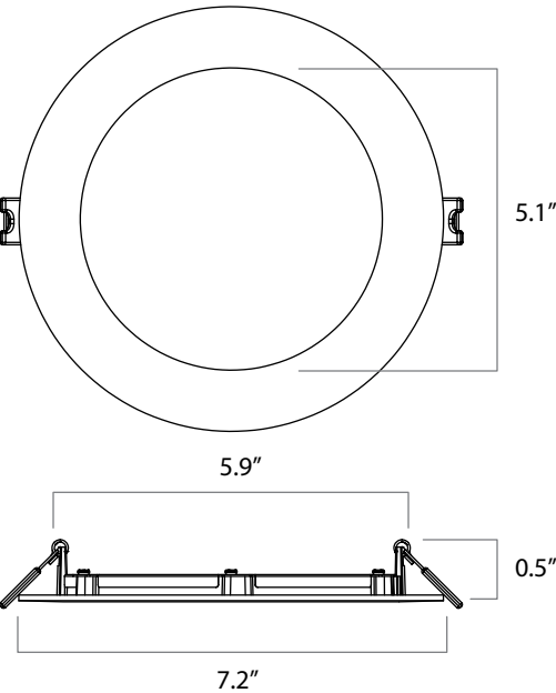
Downlight 6" Round
