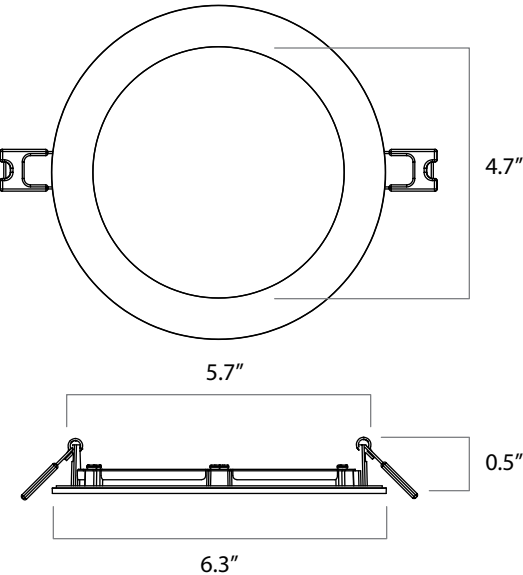
Downlight 5" Round
