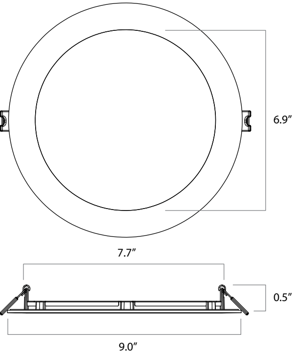
Downlight 8" Round
