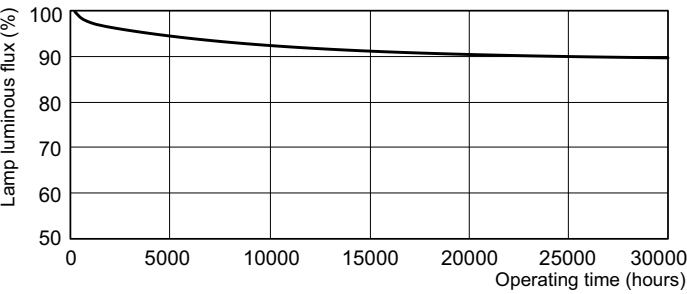
Lumen Maintenance Diagram - F54T5/865/HO/ALTO 40PK
