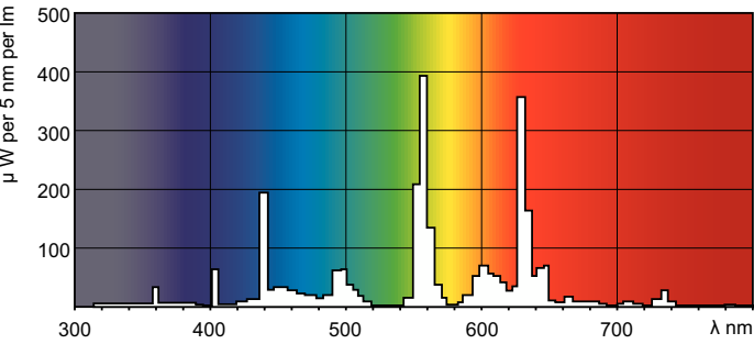
Spectral Power Distribution Colour - F54T5/841/HO/XEW/ALTO 44W
