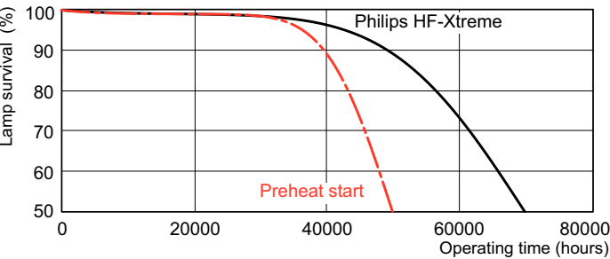
Life Expectancy Diagram - F54T5/841/HO/XEW/ALTO 44W
