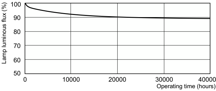
Lumen Maintenance Diagram - F54T5/841/HO/XEW/ALTO 44W
