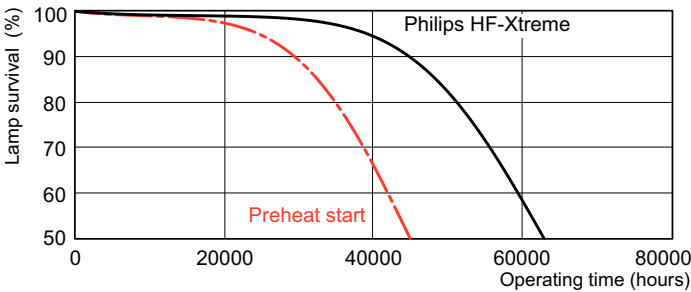
Life Expectancy Diagram - F54T5/841/HO/XEW/ALTO 44W
