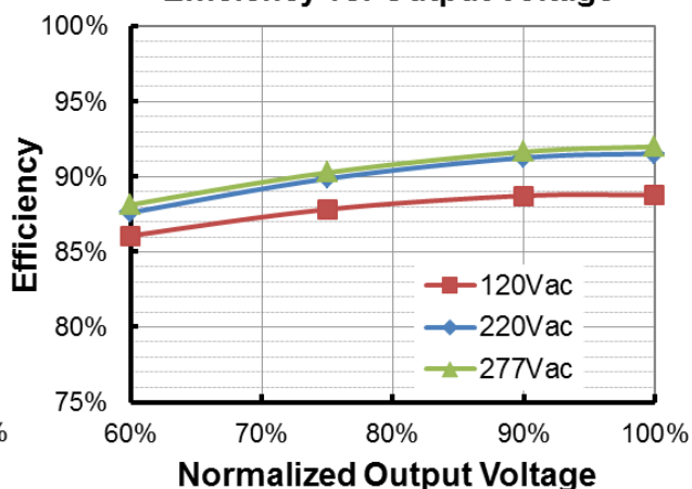
EUM-200S560DT ( I_o=5600mA ) Efficiency vs. Output Voltage
