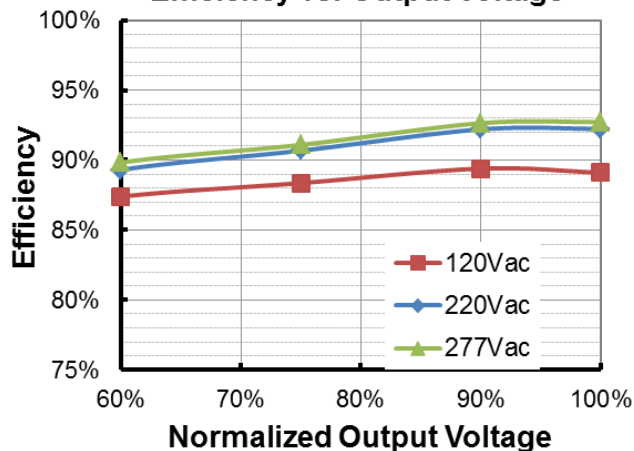
EUM-200S280DT ( I_o=2800mA ) Efficiency vs. Output Voltage
