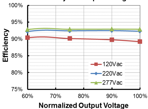
EUM-200S280DT ( I_o=1800mA ) Efficiency vs. Output Voltage
