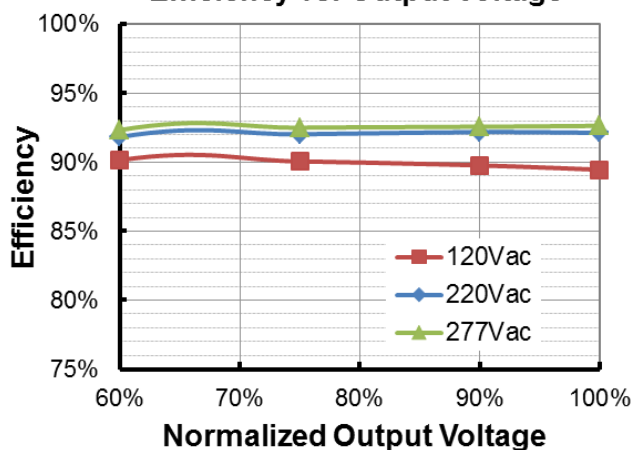
EUM-200S560DT ( I_o=3500mA ) Efficiency vs. Output Voltage
