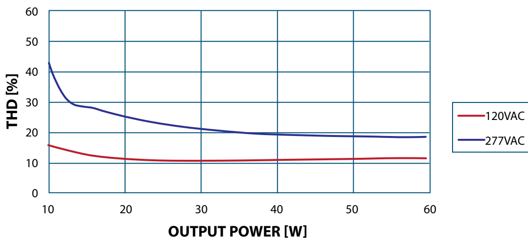
THD VS. OUTPUT POWER
