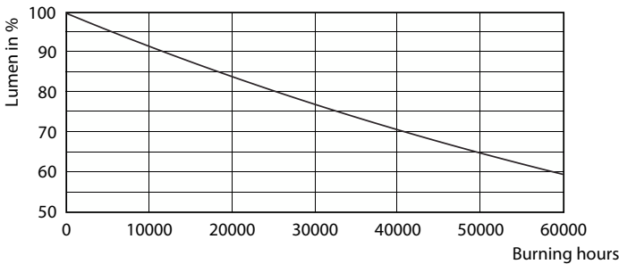
Lumen Maintenance Diagram - 12PAR30L/EXPERTCOLOR RETAIL/F25/930/DIM
