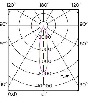
Light Distribution Diagram - 17PAR38/EXPERTCOLOR RETAIL/F25/930/DIM B
