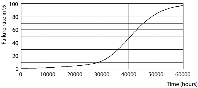
Life Expectancy Diagram - 16AR111/LED/927/F40/DIM/EC 12V 6/1FB
