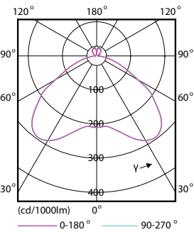
NAM Highbay 165W EX39 4000K 120D WB UDL
