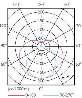
Light Distribution Diagram - 14T5HE/46-840/IF21/G/DIM 10/1
