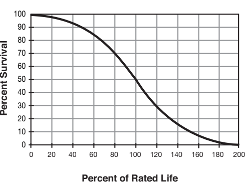
Mortality Curve
