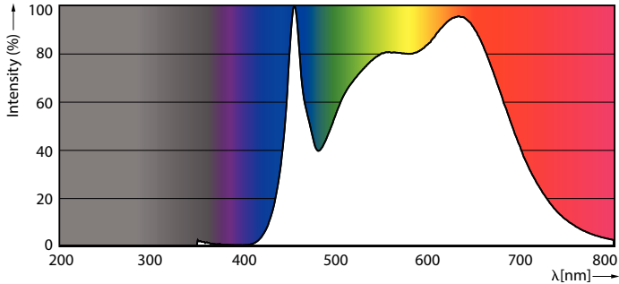
Spectral Power Distribution Colour - 14PAR38/EXPERTCOLOR/ F40/940/P/D/T20/JA8
